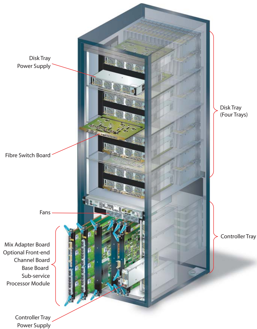
Figure 13. Rear view of an NSC55 chassis in a 42U rack.
