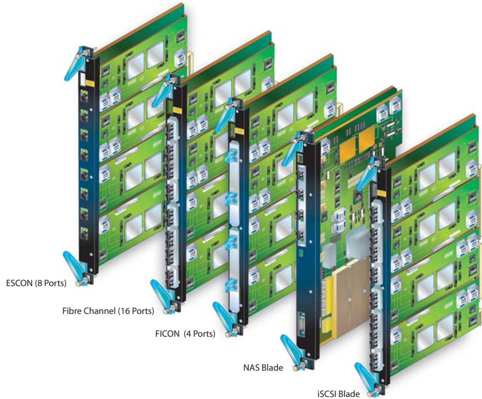
Figure 21. Fibre Channel, ESCON, and FICON front-end directors, and NAS and iSCSI Blades
