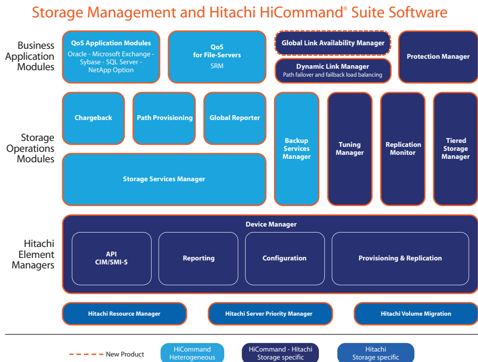
Figure 32. The framework for Storage Management and HiCommand Suite software: heterogeneous storage management software and Hitachi storage-specific management software.
