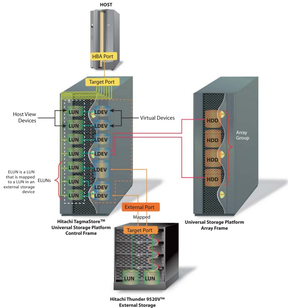
Figure 25. A host LUN is mapped through an external LUN (ELUN) in the Universal Storage Platform to a LUN in an external storage device.
