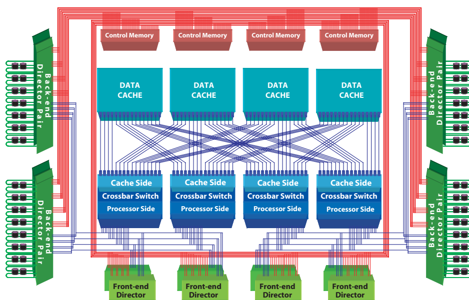
Figure 17. The Universal Storage Platform and Network Storage Controller are based on a breakthrough VLSI massively parallel crossbar switch architecture.
