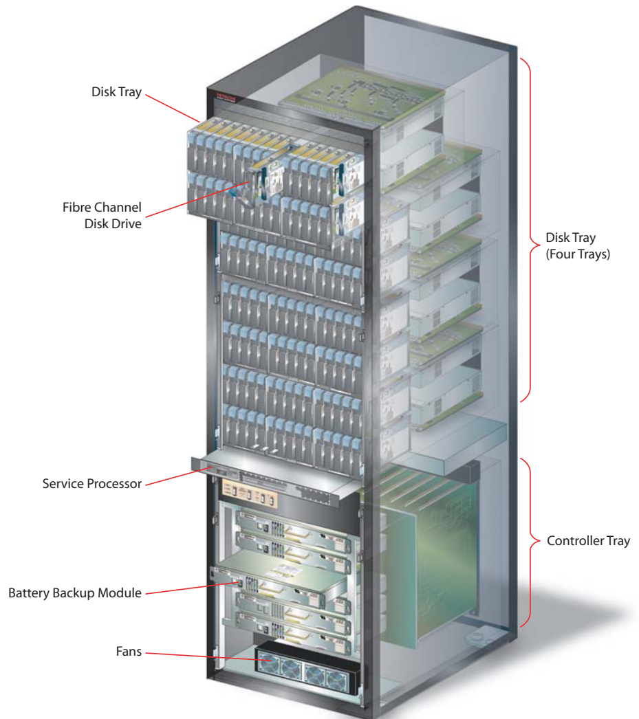
Figure 12. Front view of an NSC55 in a 42U rack.
