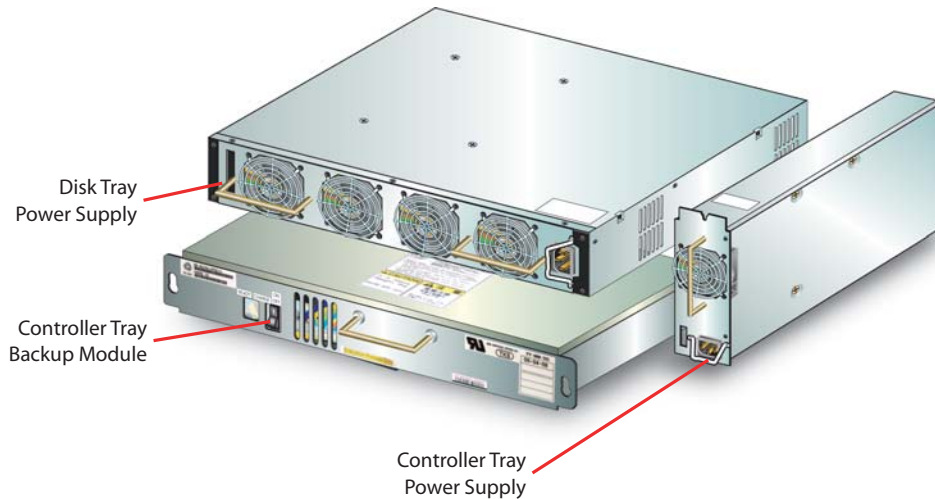
Figure 16. An NSC55 disk tray power supply, a controller tray power supply, and a backup module.
