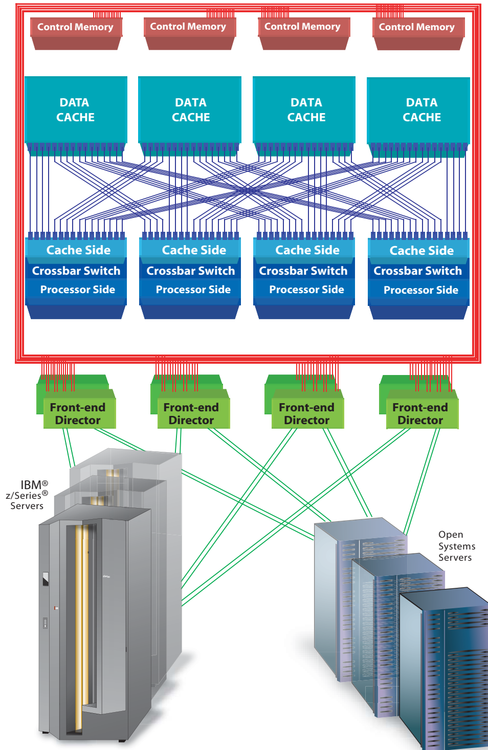
Figure 20. The Universal Storage Platform and Network Storage Controller provide Fibre Channel, ESCON, and FICON attachment to open systems and mainframe hosts.
