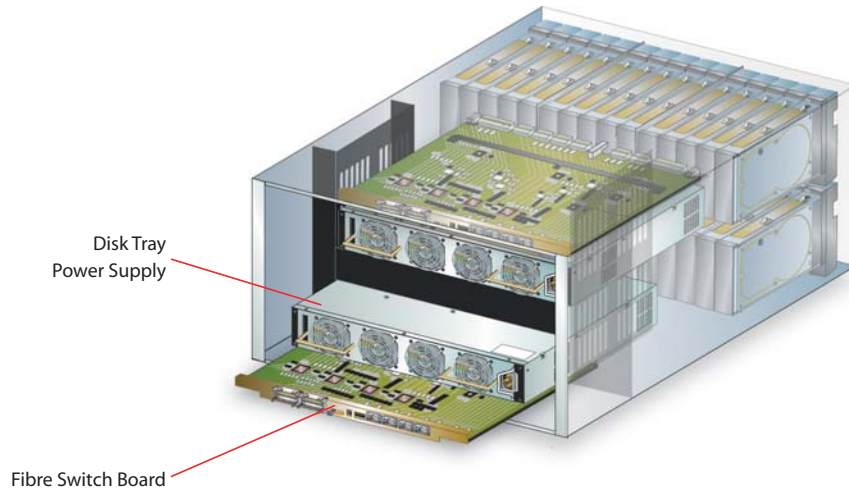
Figure 14. Rear view of an NSC55 disk tray.
