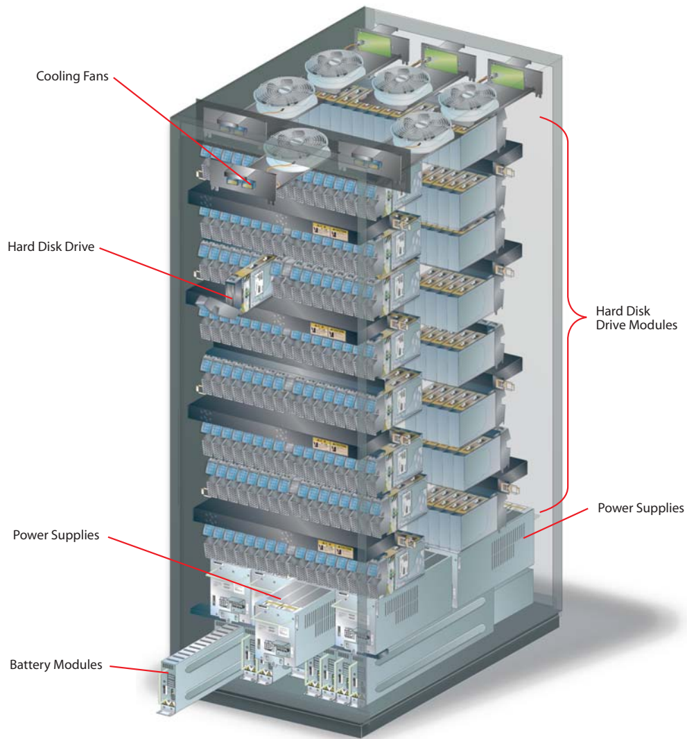
Figure 9. Universal Storage Platform model USP1100 Array Frame with its major components.
